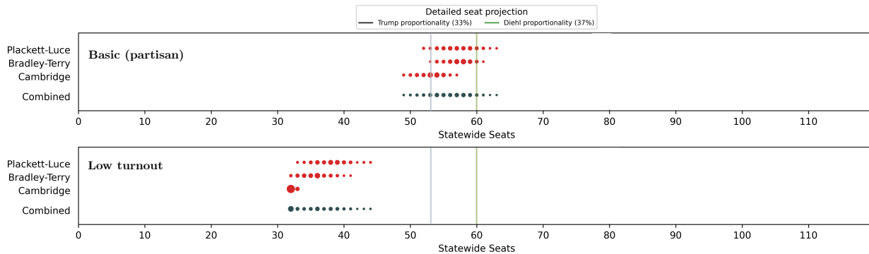
Figure 9. Projected outcomes of STV elections with partisan bloc voters, using Diehl's support in the Senate race of 2018 as the pattern of Republican voting.
