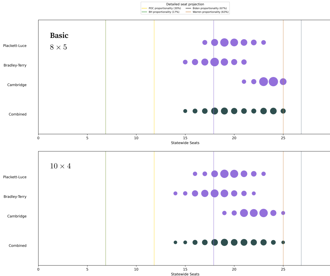
Figure 6. Top: basic, with 8 \times 5 zones. Bottom: 10 \times 4 . The projected difference between eight 5-member zones and ten 4-member zones is quite modest.
